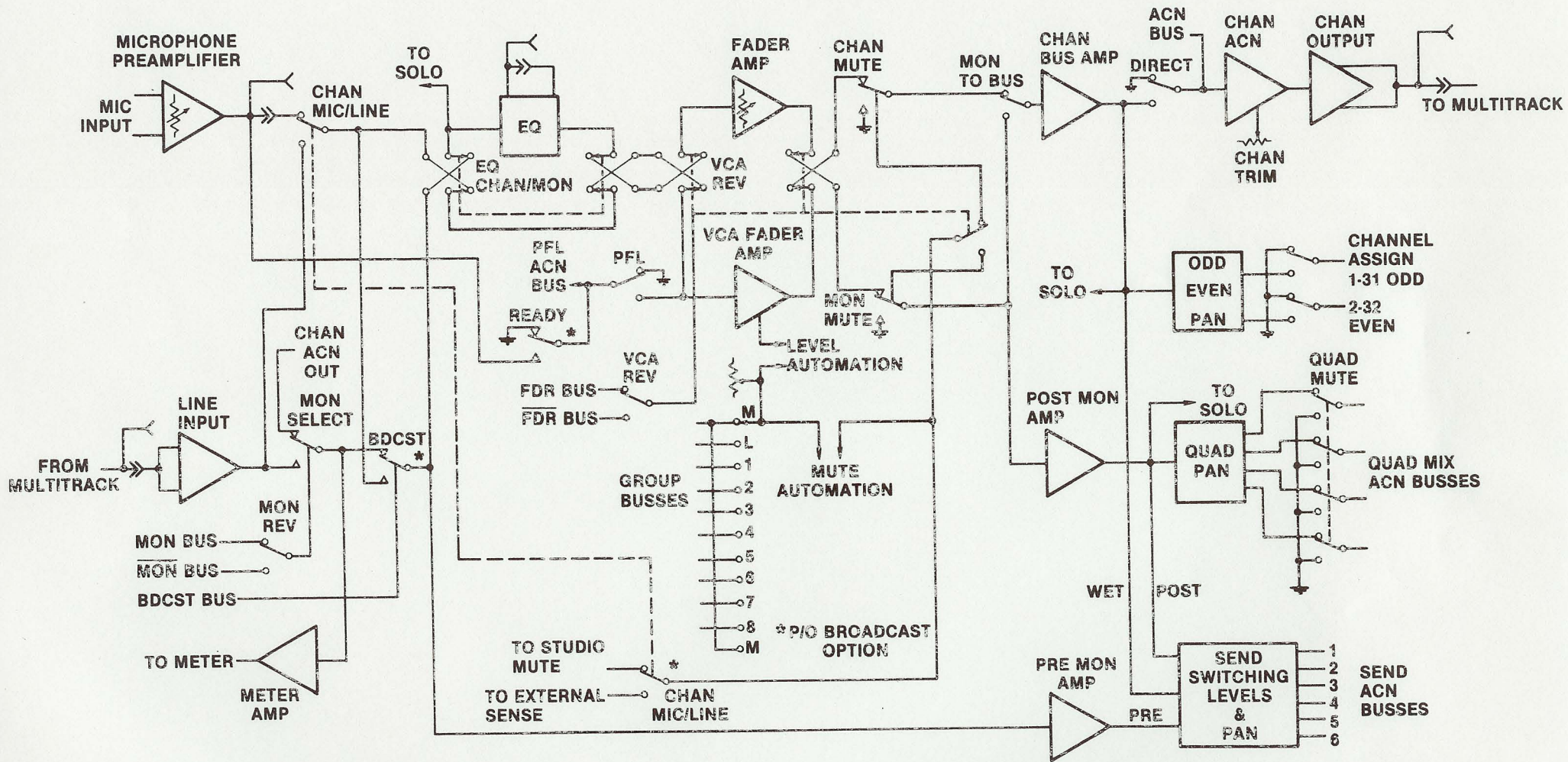
NEC JH-500D I/O SIGNAL FLOW
